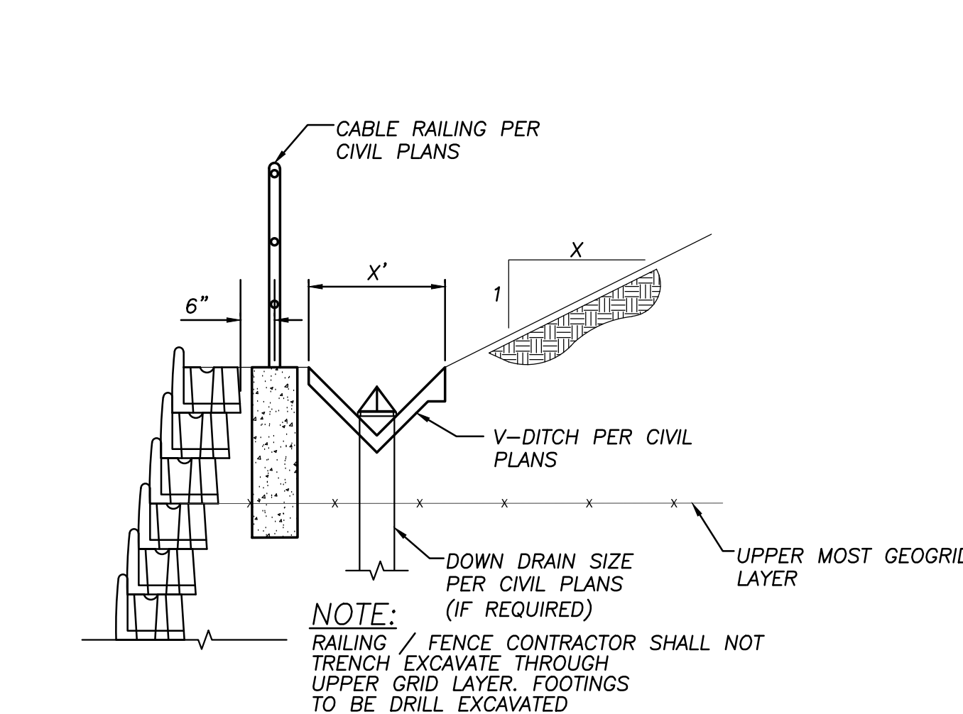
TYPICAL SLOPE CONDITION DETAIL
