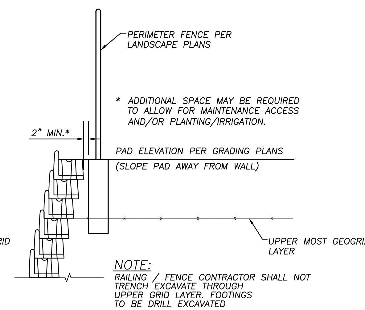
TYPICAL LEVEL CONDITION DETAIL
