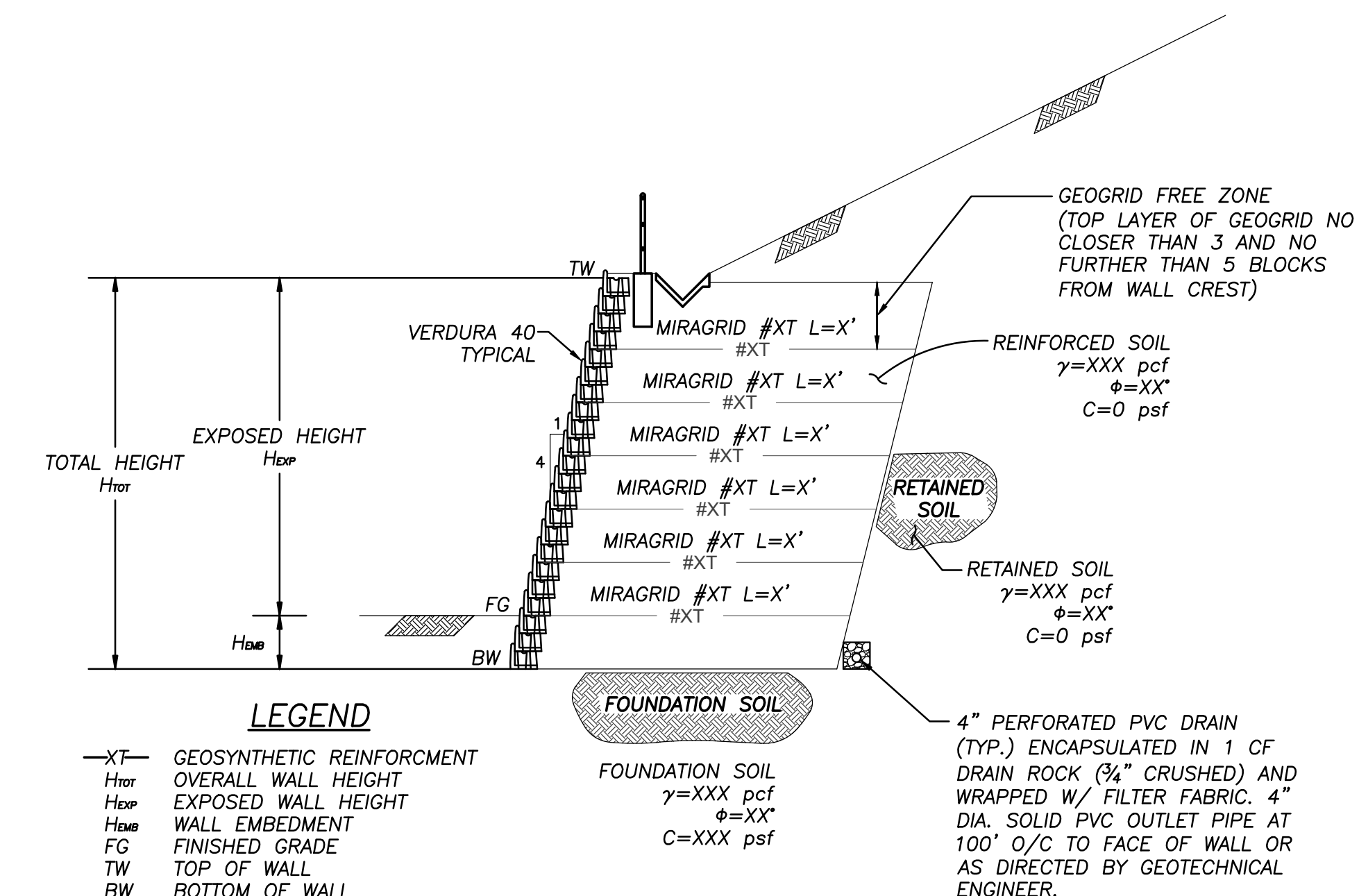
TYPICAL CROSS SECTION DETAIL
