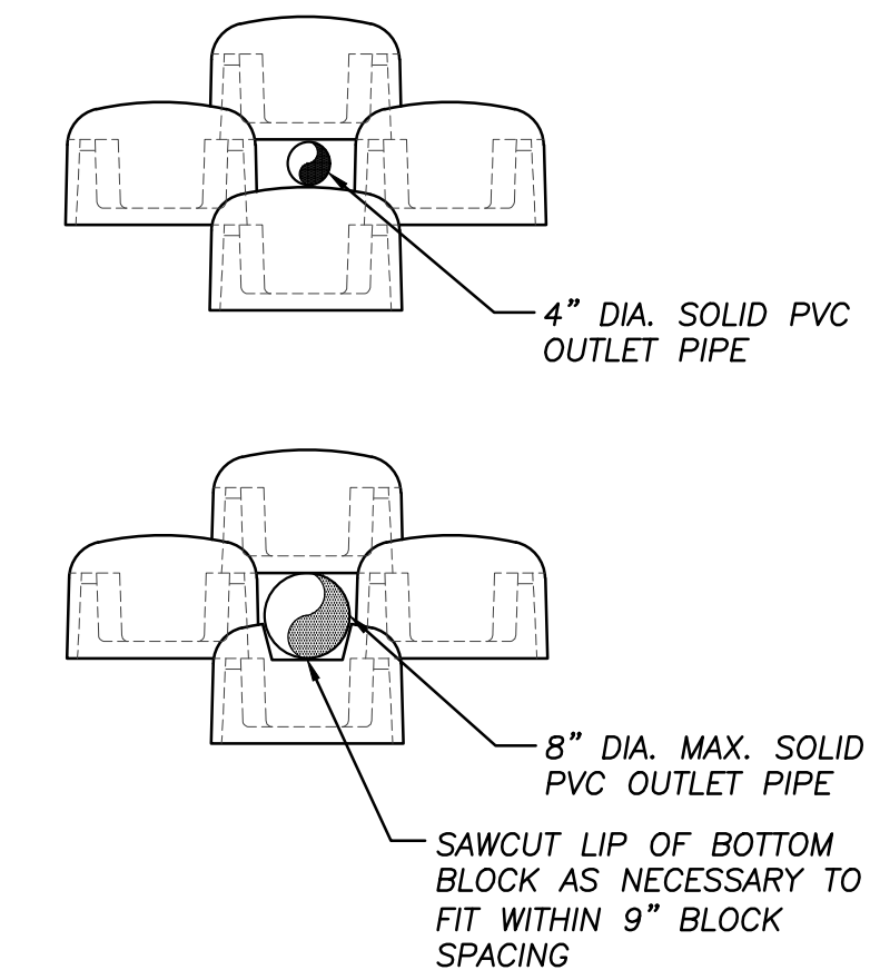
TYPICAL PENETRATION DETAIL
